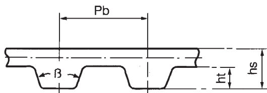
Metric T Type Synchronous Belt
