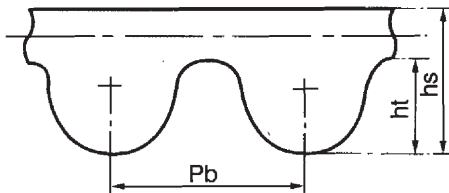
HTD ARC TOOTH
