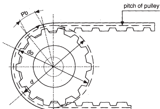
Schematic drawing of synchronous pulley
