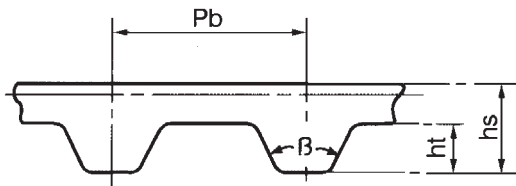
Inch T Type Synchronous Belt
