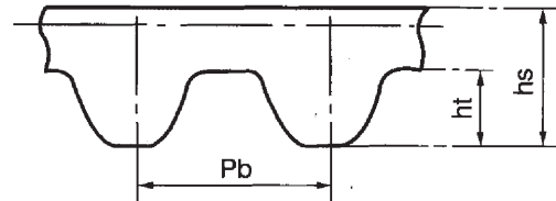
STPD/STS ARC TOOTH
